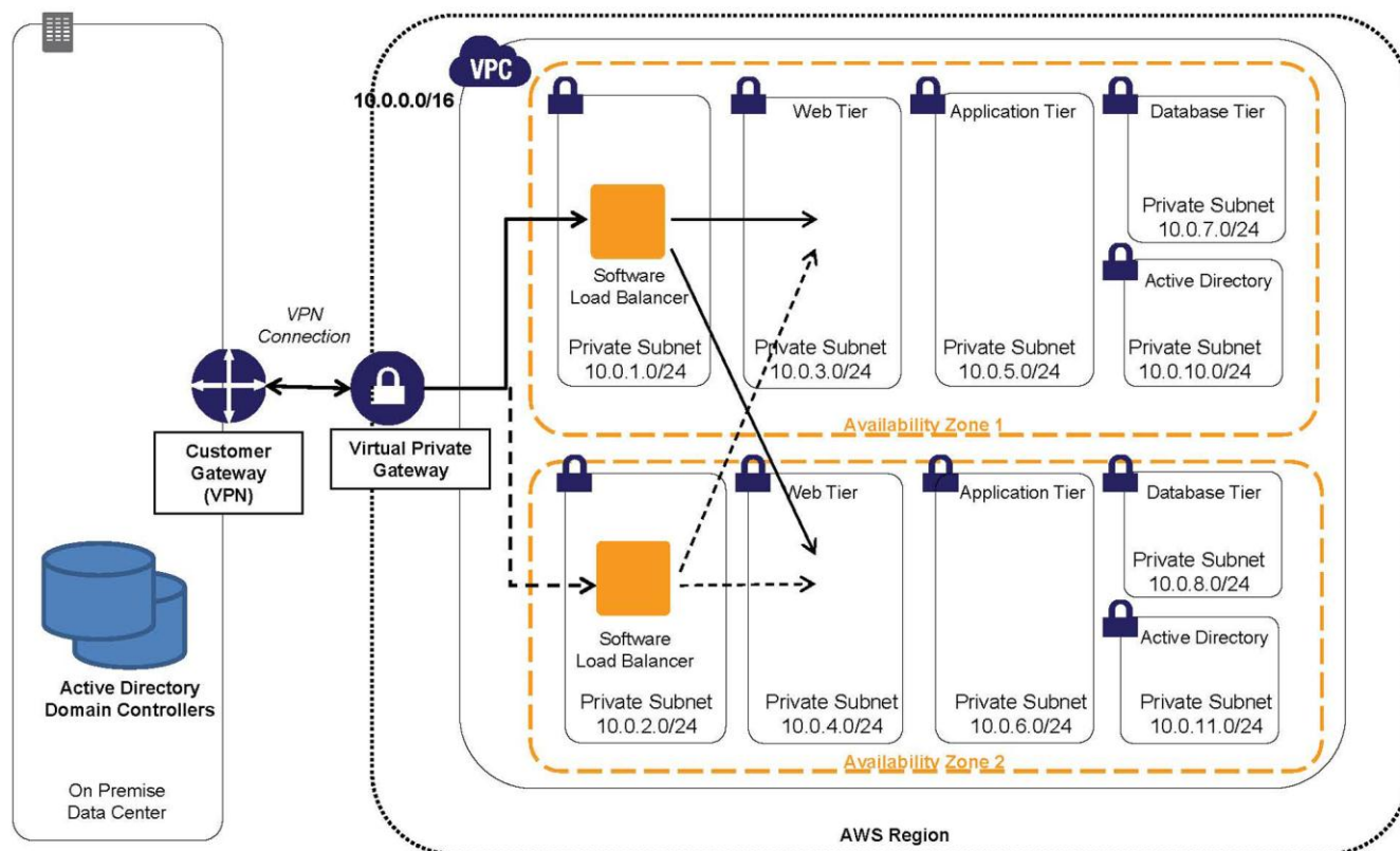
Figure 4: Network configuration for the intranet scenario
