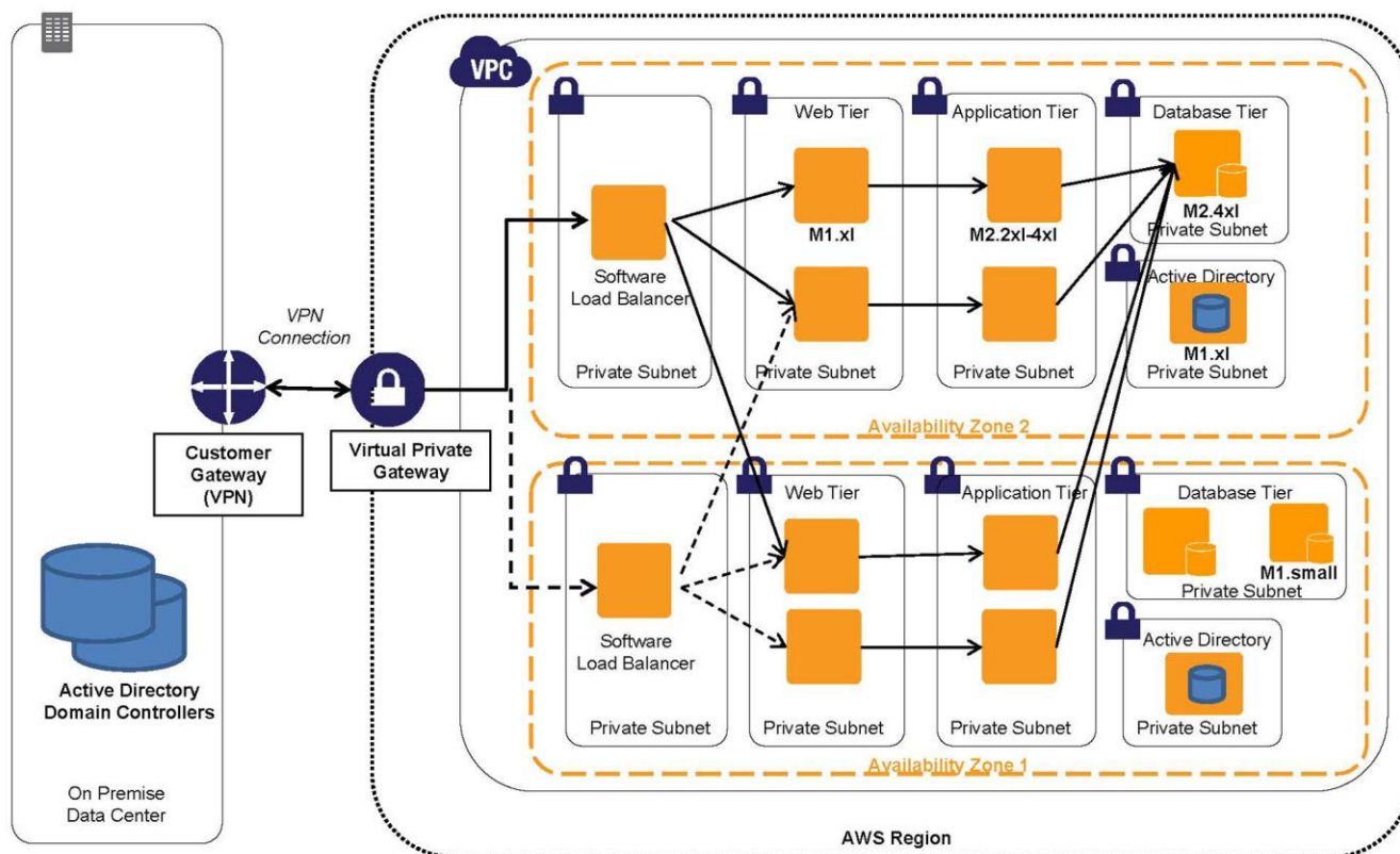
Figure 12: Intranet SharePoint Server farm in AWS
